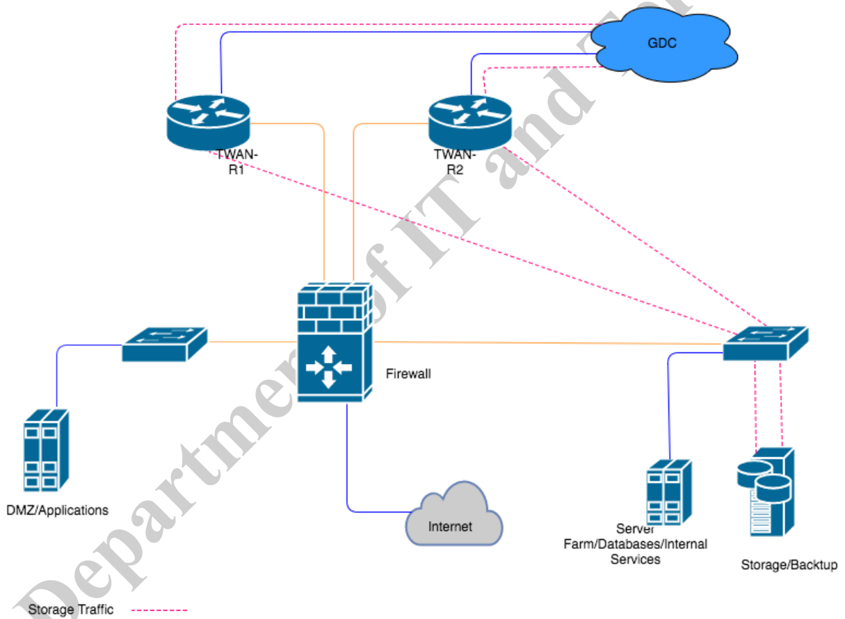
Figure: Network Diagram [GDC Backup Site]
